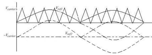
Fig.1 Carrier and Reference Signals.
