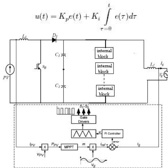
Fig. 4 . 13-level inverter with PI controller
