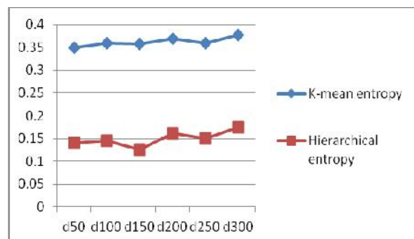
Fig.4: Entropy comparison of k-mean and hierarchical
