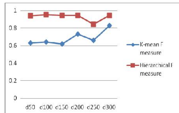
Fig.3: f measure comparison of k-mean and hierarchical
