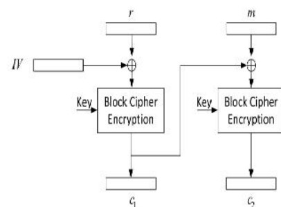
Fig. 2. The Cipher Block Chaining (CBC) mode of encryption used for message encryption. The random number, r ,
