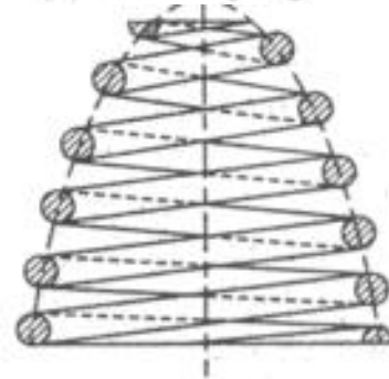
(b) Volute spring.
