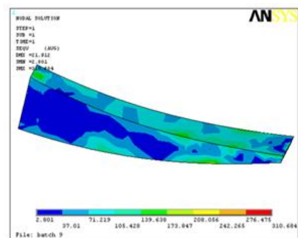
Fig-4.5: VON MISES STRESS OF COMPOSITE LEAF SPRING
