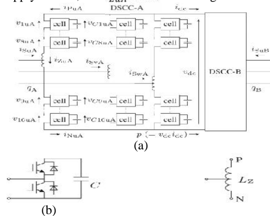
Fig 2 Circuit configuration of the DSCC-based BTB system with 16 chopper cells per leg. (a) Main circuit. (b) Chopper cell. (c) Center-tapped inductor.
