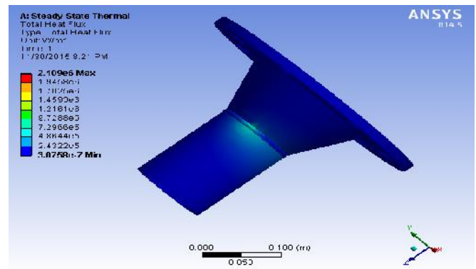
Fig9 Total heat flux of directed welded stainless steel pipe
