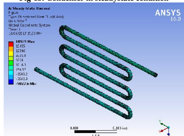
Fig-16: condenser out let min, max temperature values
