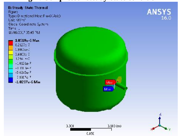
Fig-5: Compressor out let temperature min, max values
